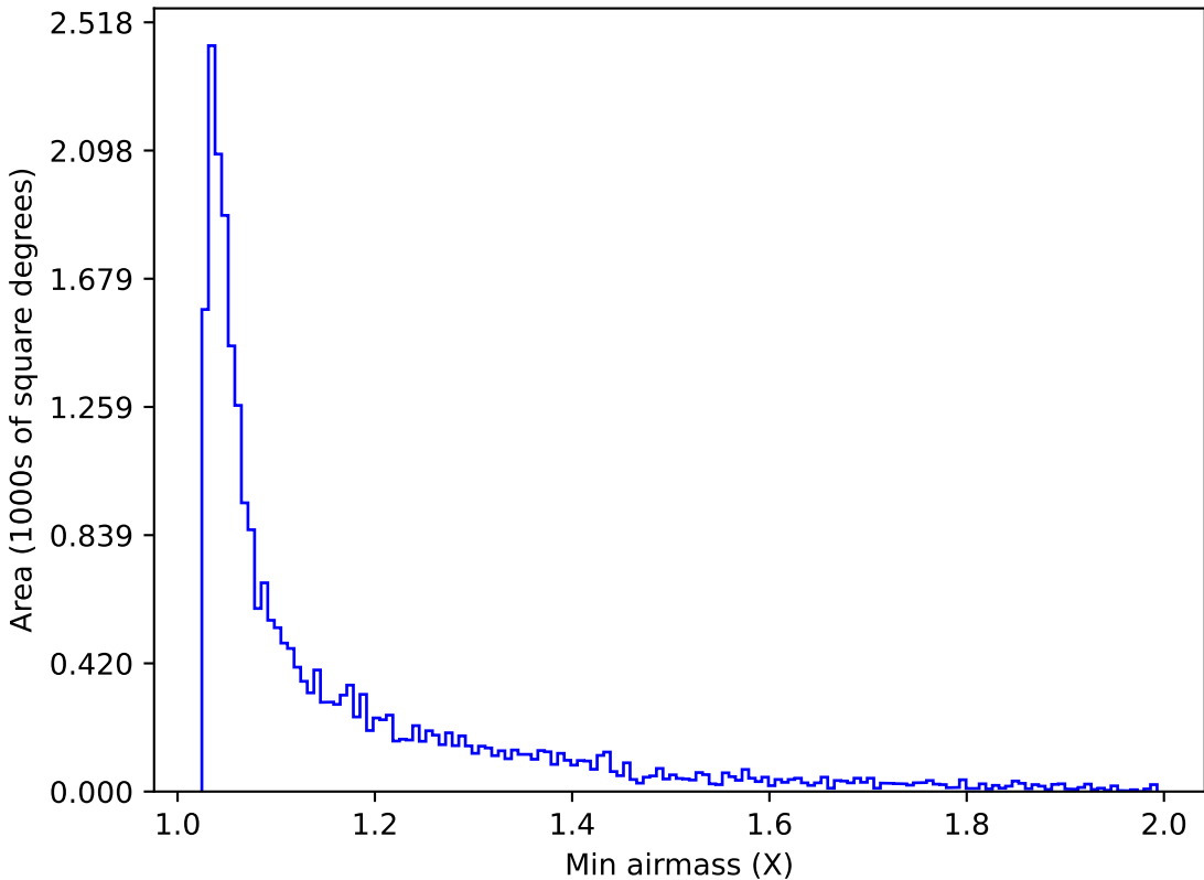
too_elab_r8_d2_gz_v3.4_10yrs Yr 1 z band: Min airmass
