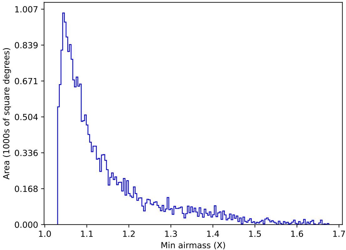
too_elab_r8_d2_gz_v3.4_10yrs Yr 1 u band: Min airmass
