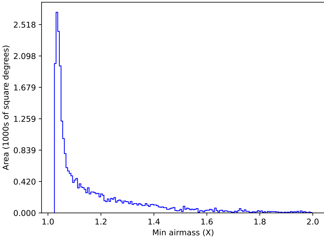
too_elab_r8_d2_gz_v3.4_10yrs Yr 1 r band: Min airmass
