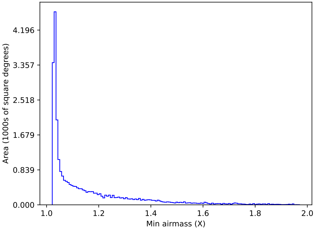
too_elab_r8_d2_gz_v3.4_10yrs Yr 1 all bands: Min airmass
