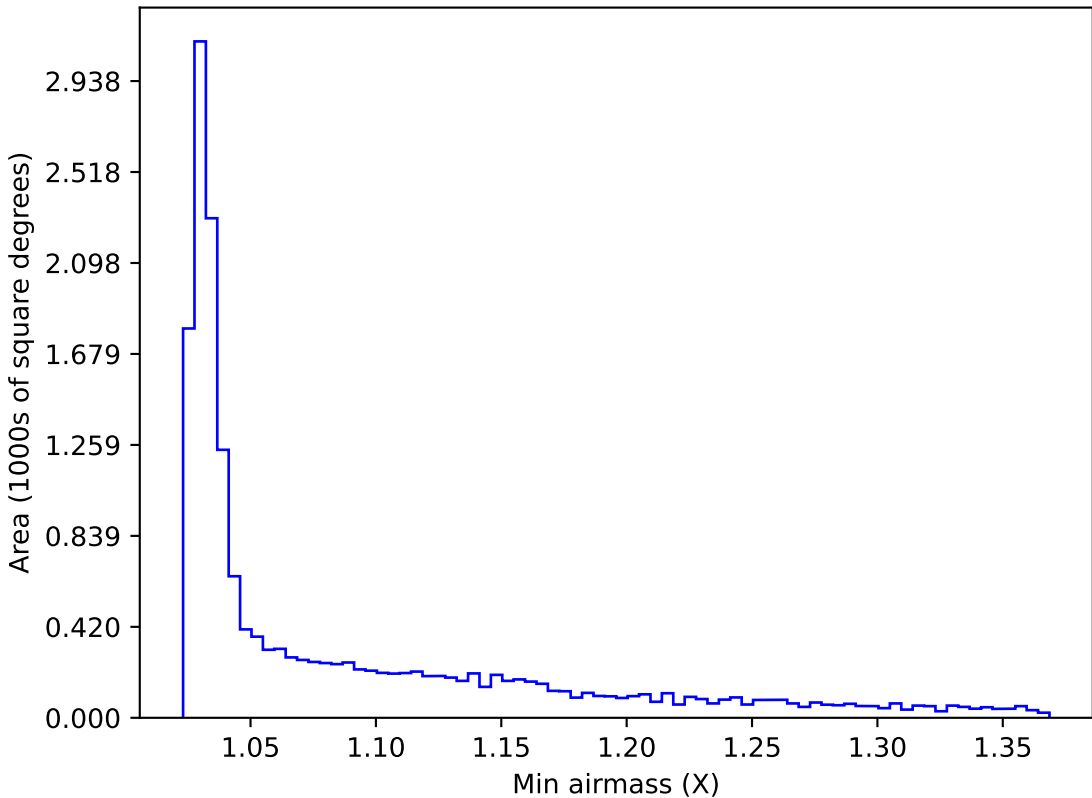
too_elab_r8_d2_gz_v3.4_10yrs WFD y band: Min airmass
