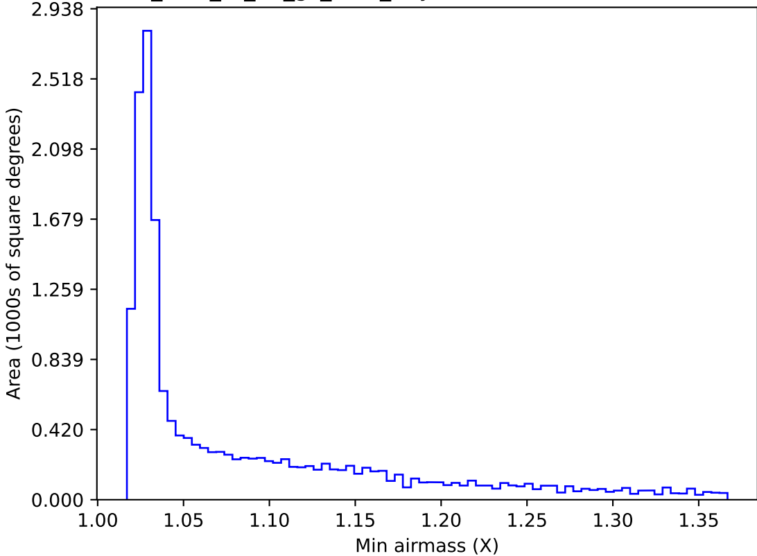
too_elab_r8_d2_gz_v3.4_10yrs WFD r band: Min airmass
