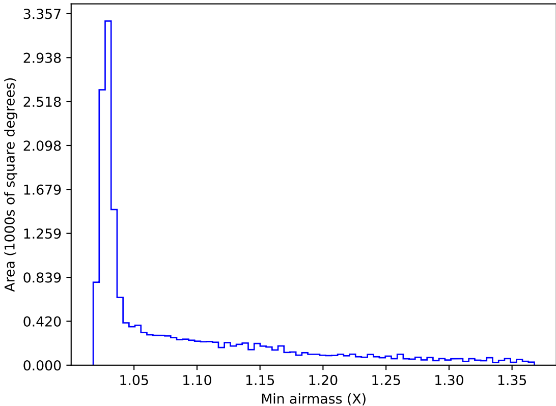
too_elab_r8_d2_gz_v3.4_10yrs WFD i band: Min airmass
