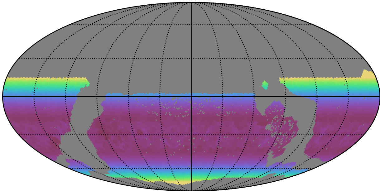
too_elab_r8_d2_gz_v3.4_10yrs WFD g band: Min airmass
