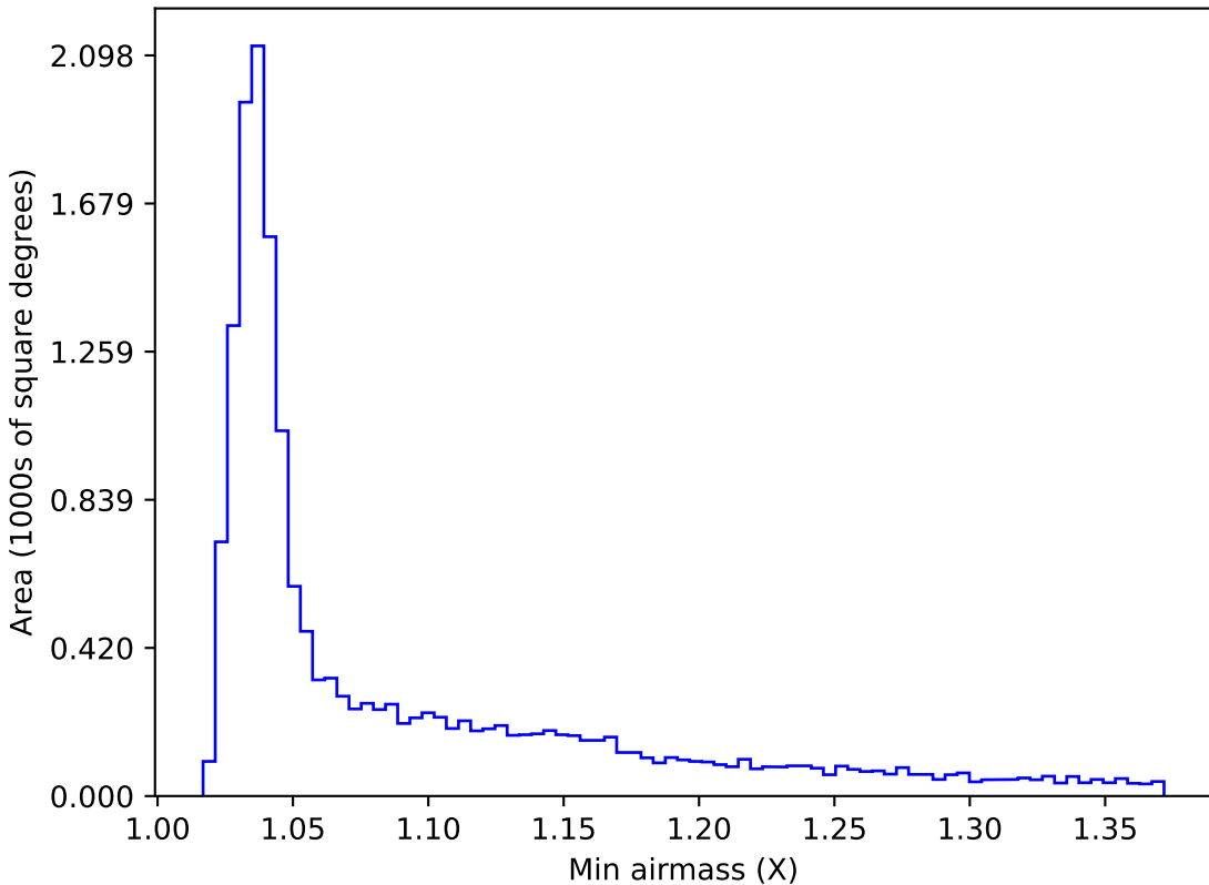
too_elab_r8_d2_gz_v3.4_10yrs WFD g band: Min airmass
