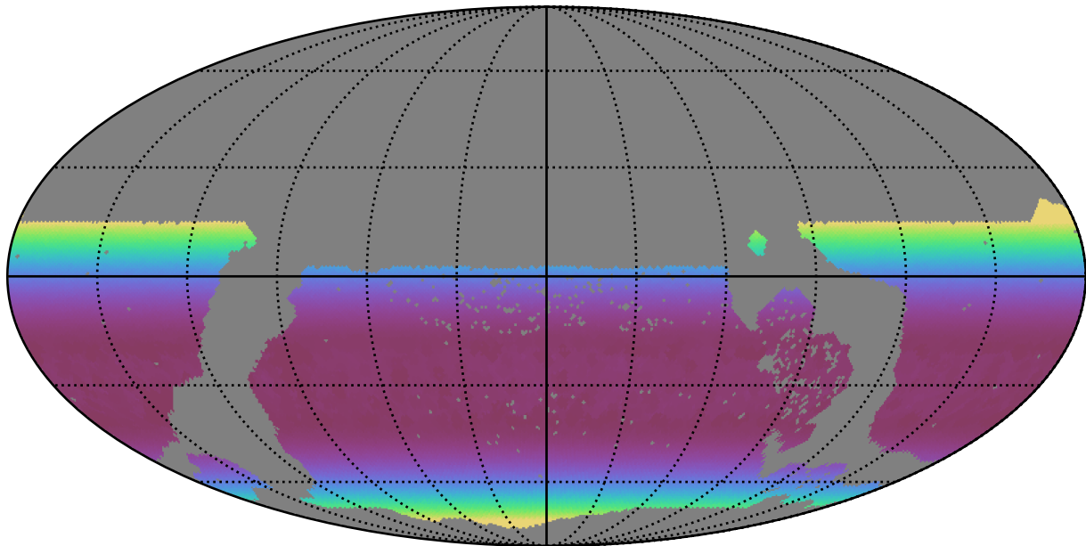
too_elab_r8_d2_gz_v3.4_10yrs WFD all bands: Min airmass
