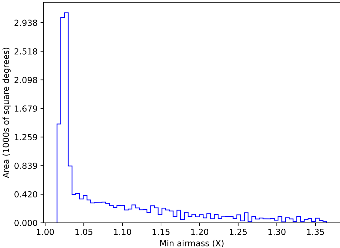
too_elab_r8_d2_gz_v3.4_10yrs WFD all bands: Min airmass
