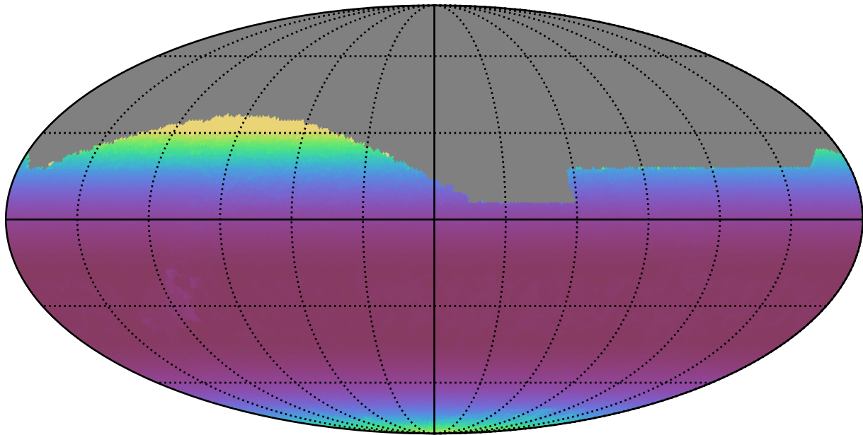
too_elab_r8_d2_gz_v3.4_10yrs All sky z band: Min airmass
