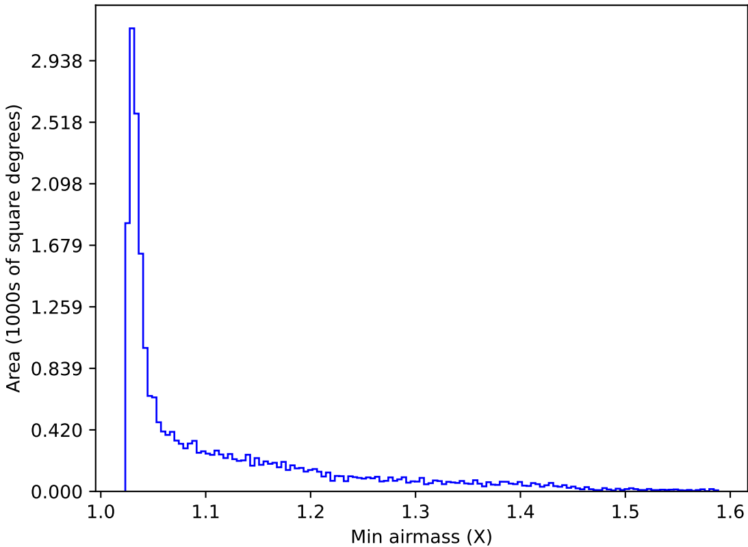
too_elab_r8_d2_gz_v3.4_10yrs All sky y band: Min airmass
