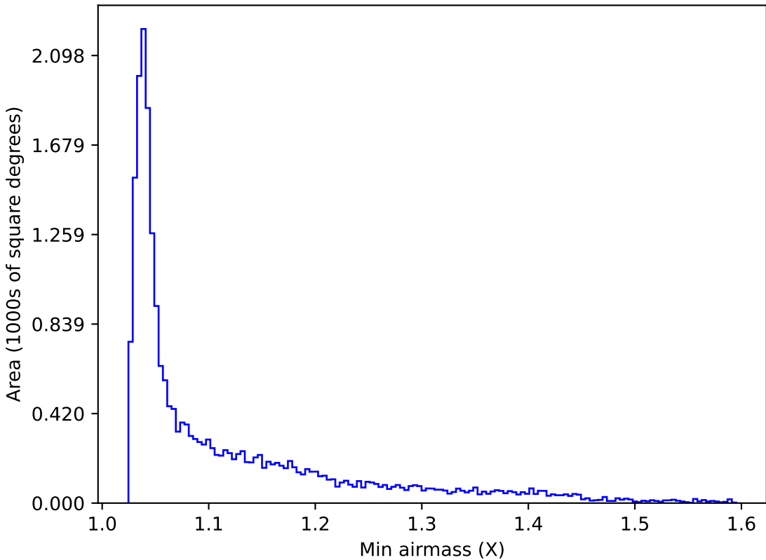
too_elab_r8_d2_gz_v3.4_10yrs All sky u band: Min airmass
