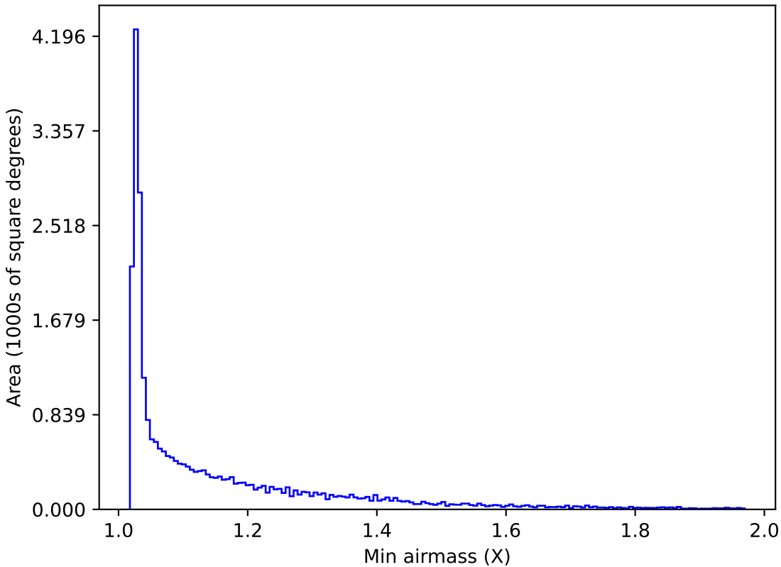
too_elab_r8_d2_gz_v3.4_10yrs All sky r band: Min airmass
