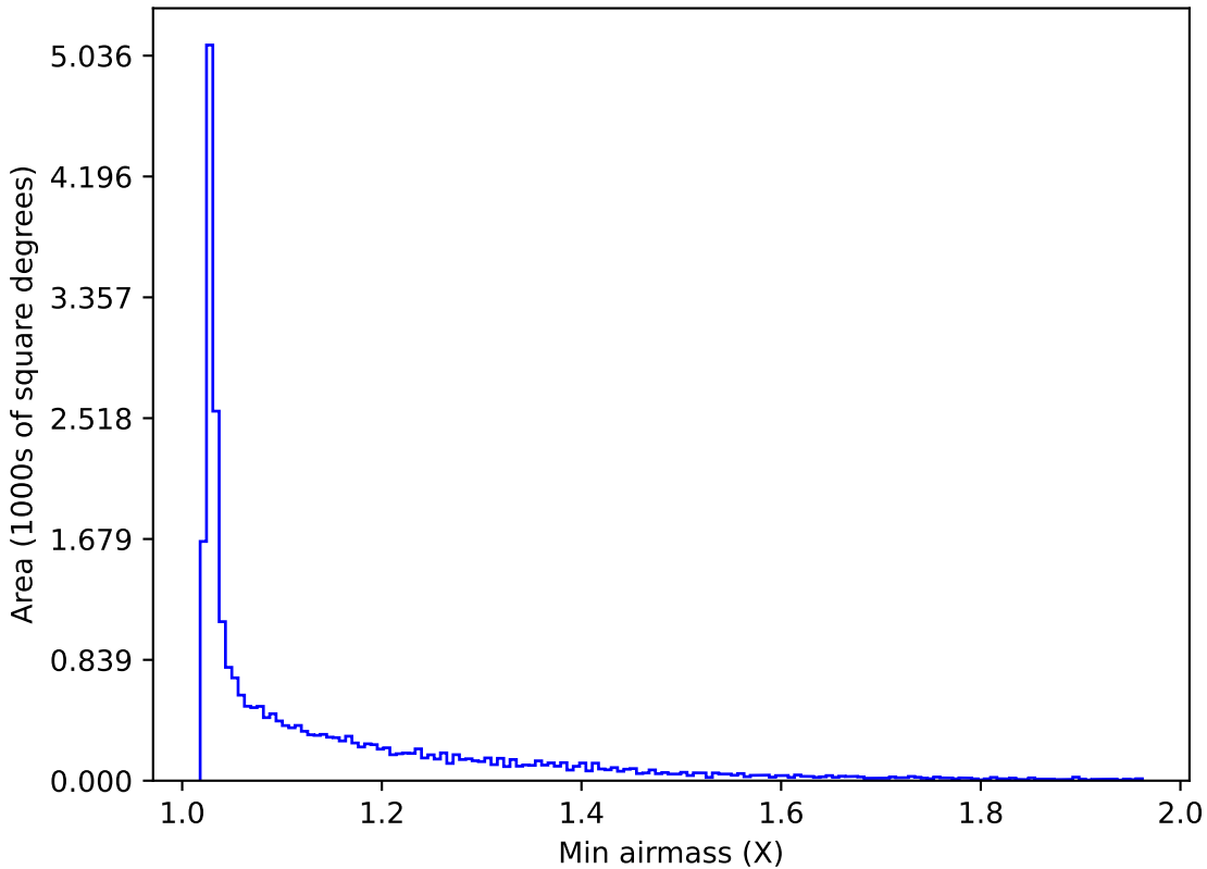
too_elab_r8_d2_gz_v3.4_10yrs All sky i band: Min airmass
