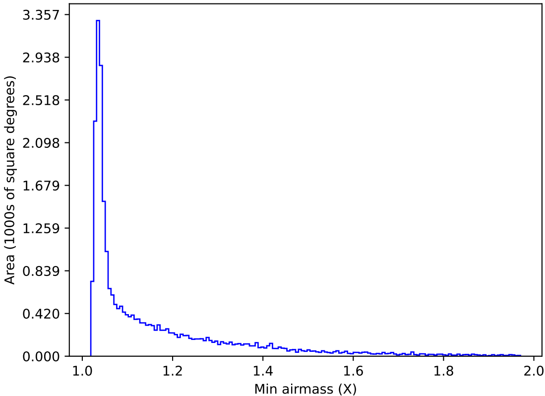
too_elab_r8_d2_gz_v3.4_10yrs All sky g band: Min airmass
