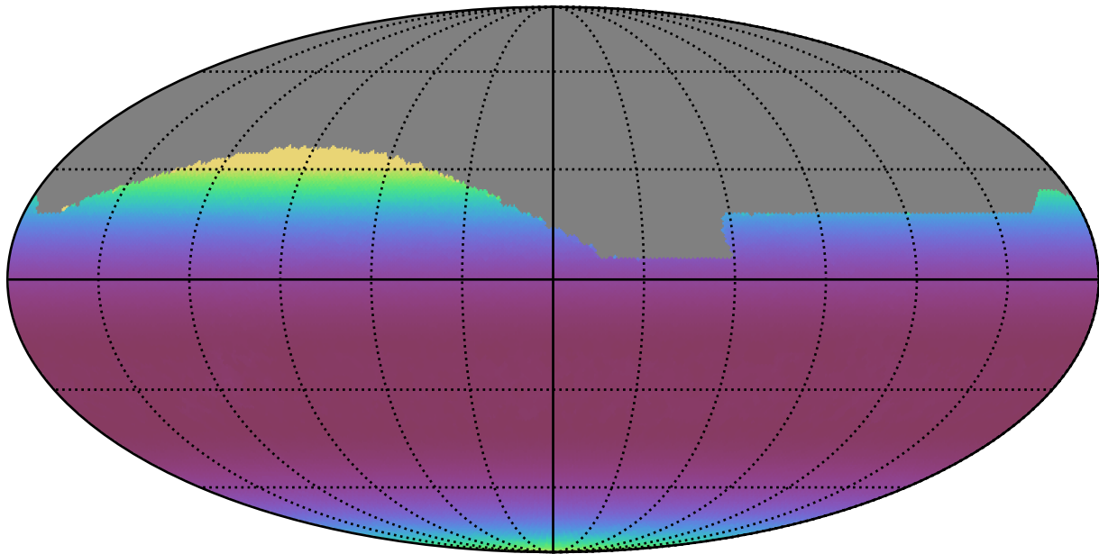
too_elab_r8_d2_gz_v3.4_10yrs All sky all bands: Min airmass
