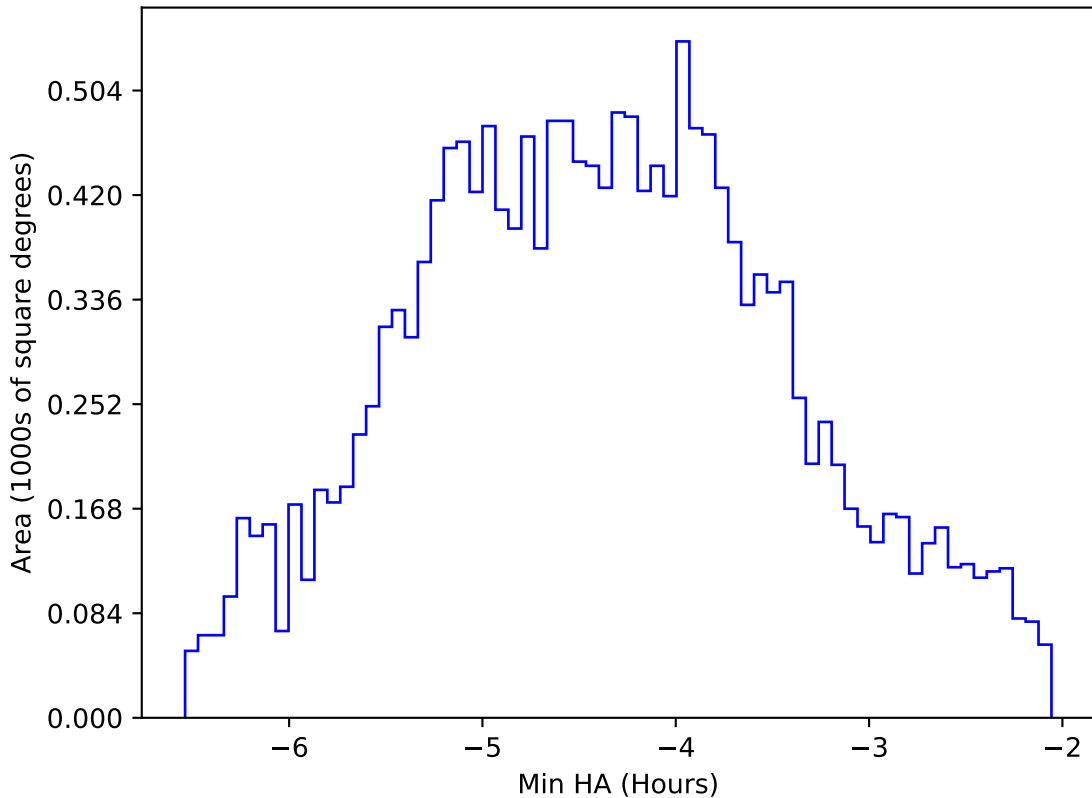
too_elab_r8_d2_gz_v3.4_10yrs WFD z band: Min HA
