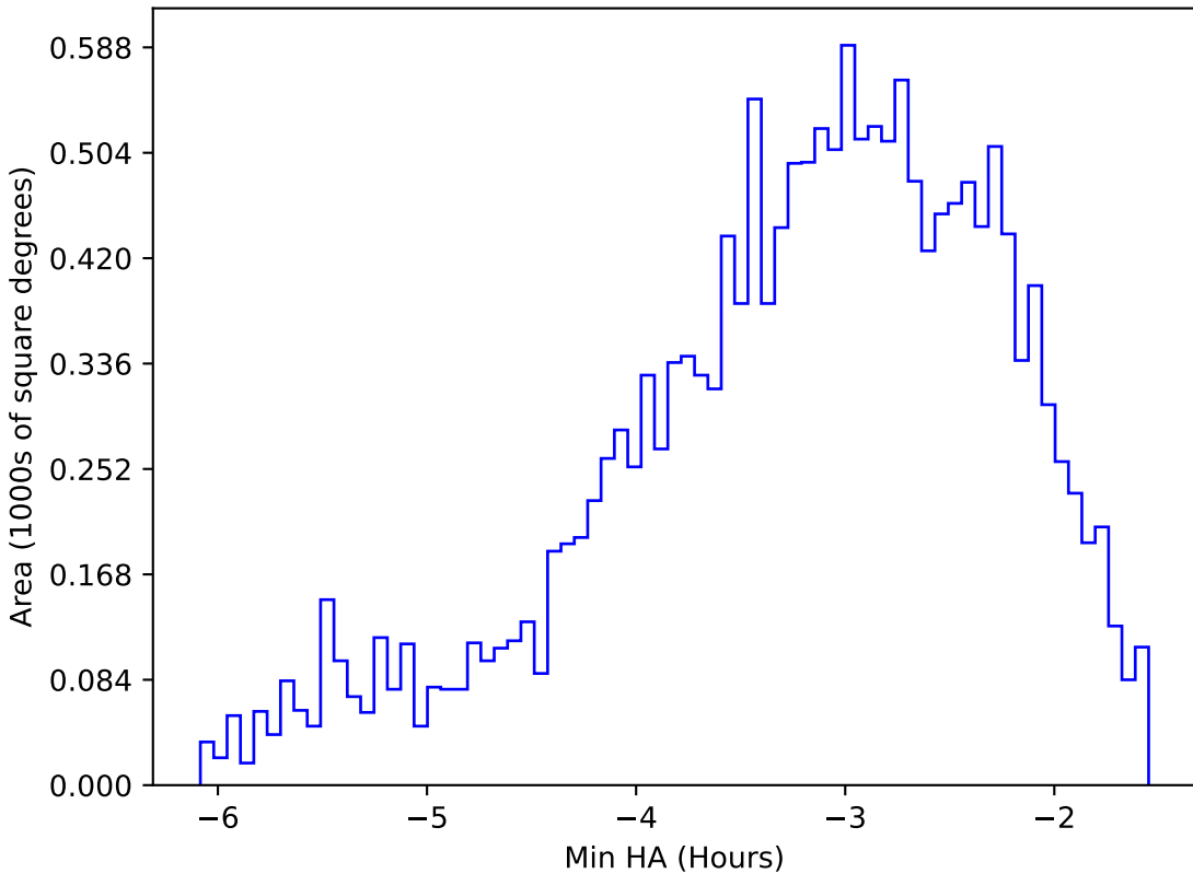
too_elab_r8_d2_gz_v3.4_10yrs WFD u band: Min HA
