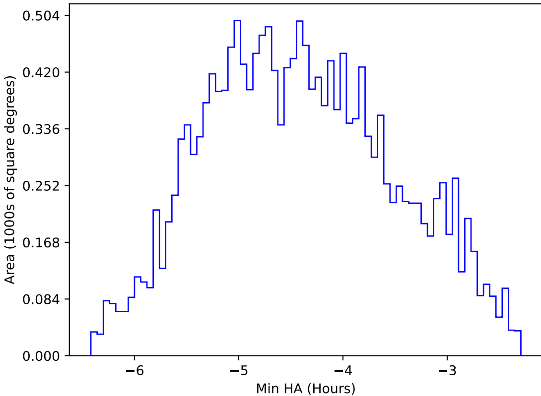
too_elab_r8_d2_gz_v3.4_10yrs WFD r band: Min HA
