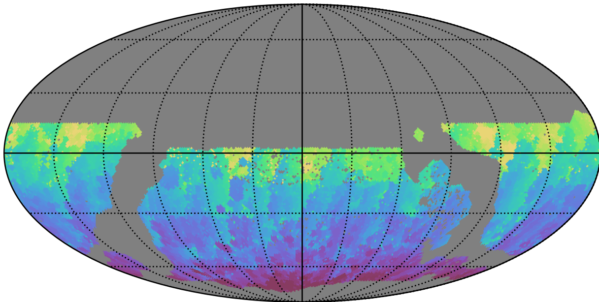
too_elab_r8_d2_gz_v3.4_10yrs WFD g band: Min HA
