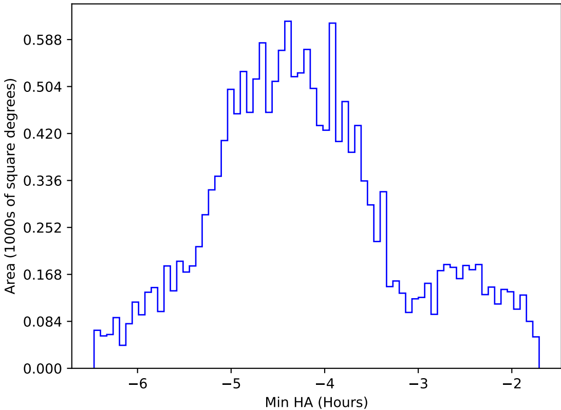
too_elab_r8_d2_gz_v3.4_10yrs WFD g band: Min HA
