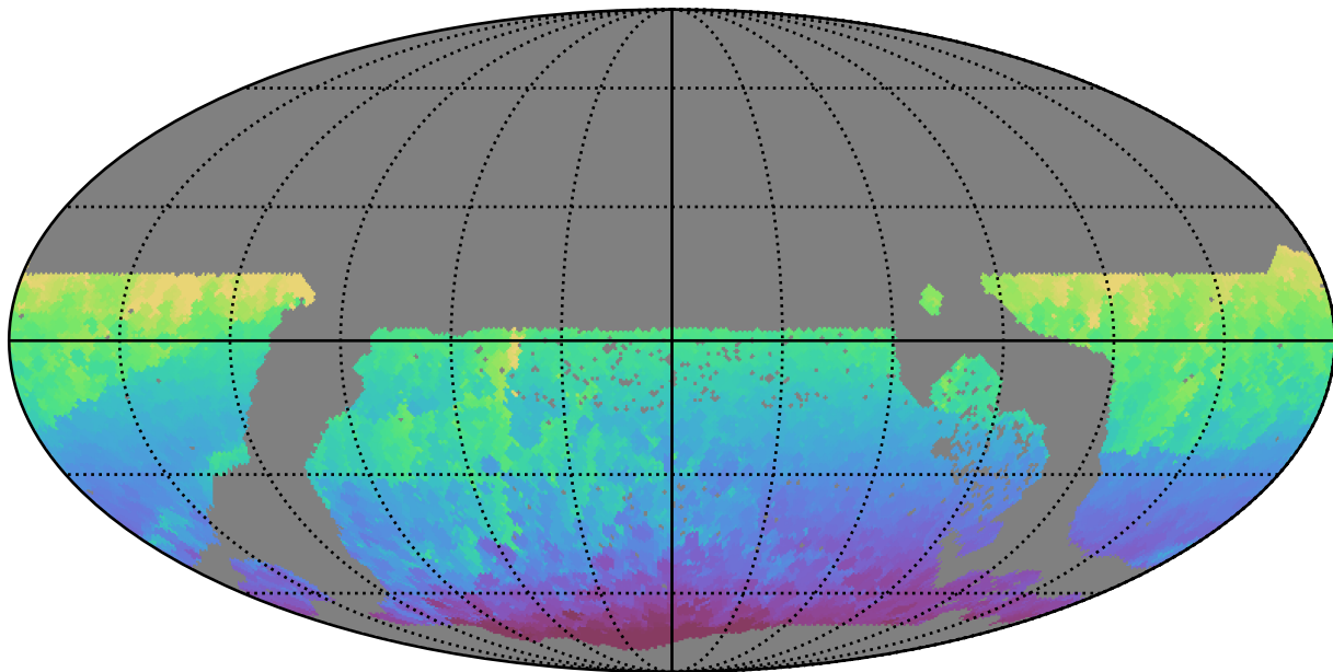
too_elab_r8_d2_gz_v3.4_10yrs WFD all bands: Min HA
