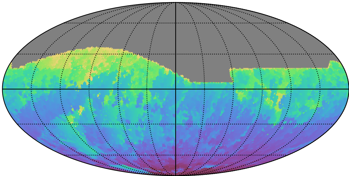
too_elab_r8_d2_gz_v3.4_10yrs All sky z band: Min HA
