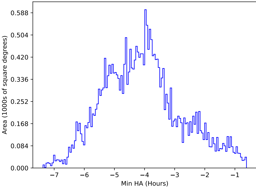
too_elab_r8_d2_gz_v3.4_10yrs All sky z band: Min HA
