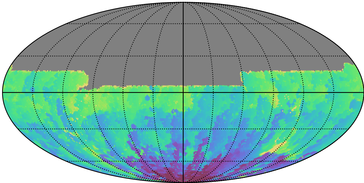
too_elab_r8_d2_gz_v3.4_10yrs All sky u band: Min HA
