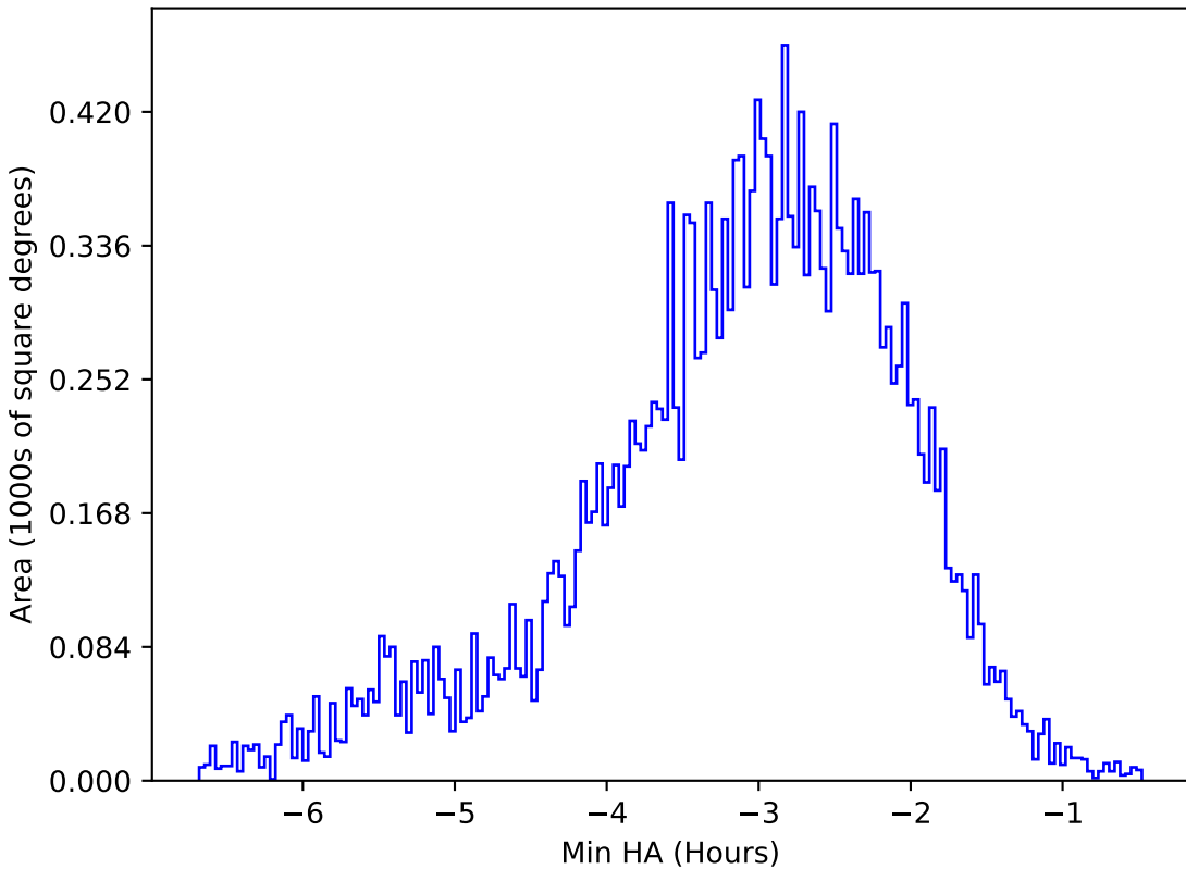
too_elab_r8_d2_gz_v3.4_10yrs All sky u band: Min HA
