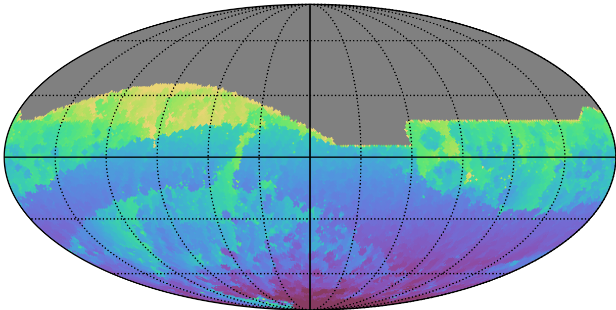
too_elab_r8_d2_gz_v3.4_10yrs All sky r band: Min HA
