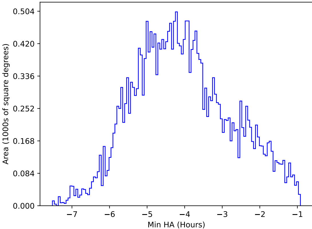
too_elab_r8_d2_gz_v3.4_10yrs All sky i band: Min HA
