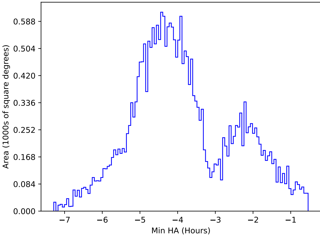
too_elab_r8_d2_gz_v3.4_10yrs All sky g band: Min HA
