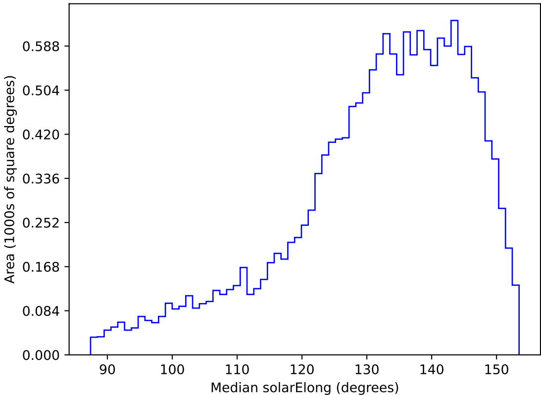
too_elab_r8_d2_gz_v3.4_10yrs WFD u band: Median solarElong
