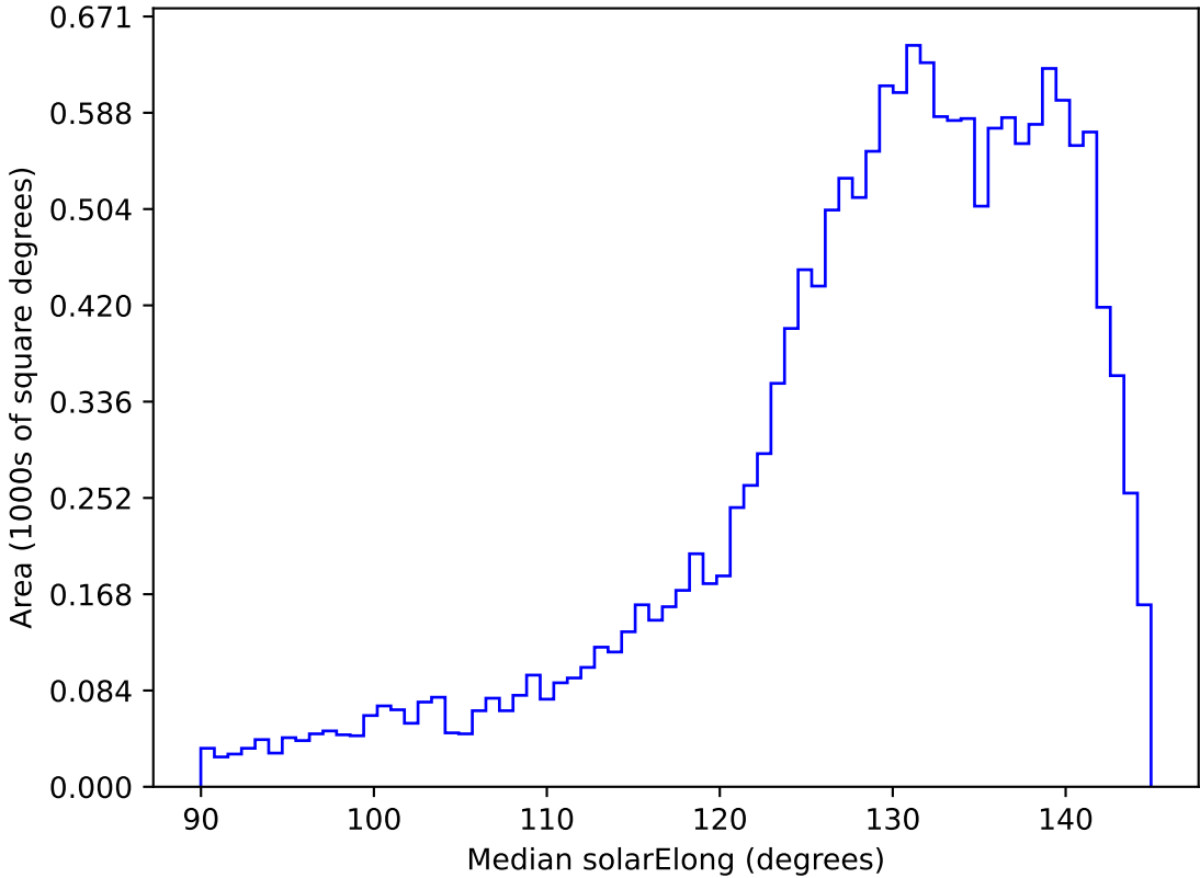
too_elab_r8_d2_gz_v3.4_10yrs WFD i band: Median solarElong
