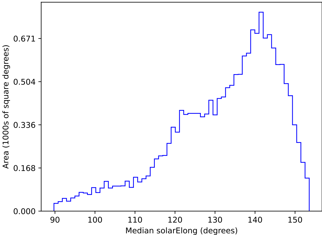
too_elab_r8_d2_gz_v3.4_10yrs WFD g band: Median solarElong
