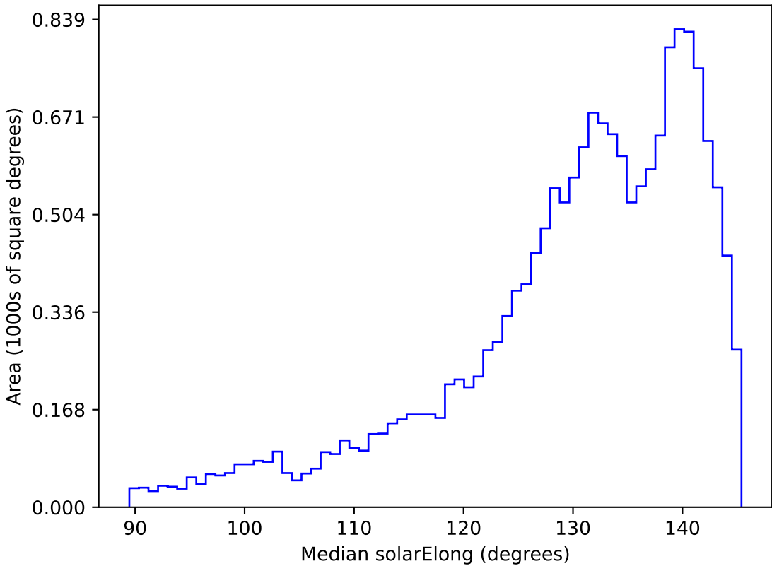
too_elab_r8_d2_gz_v3.4_10yrs WFD all bands: Median solarElong
