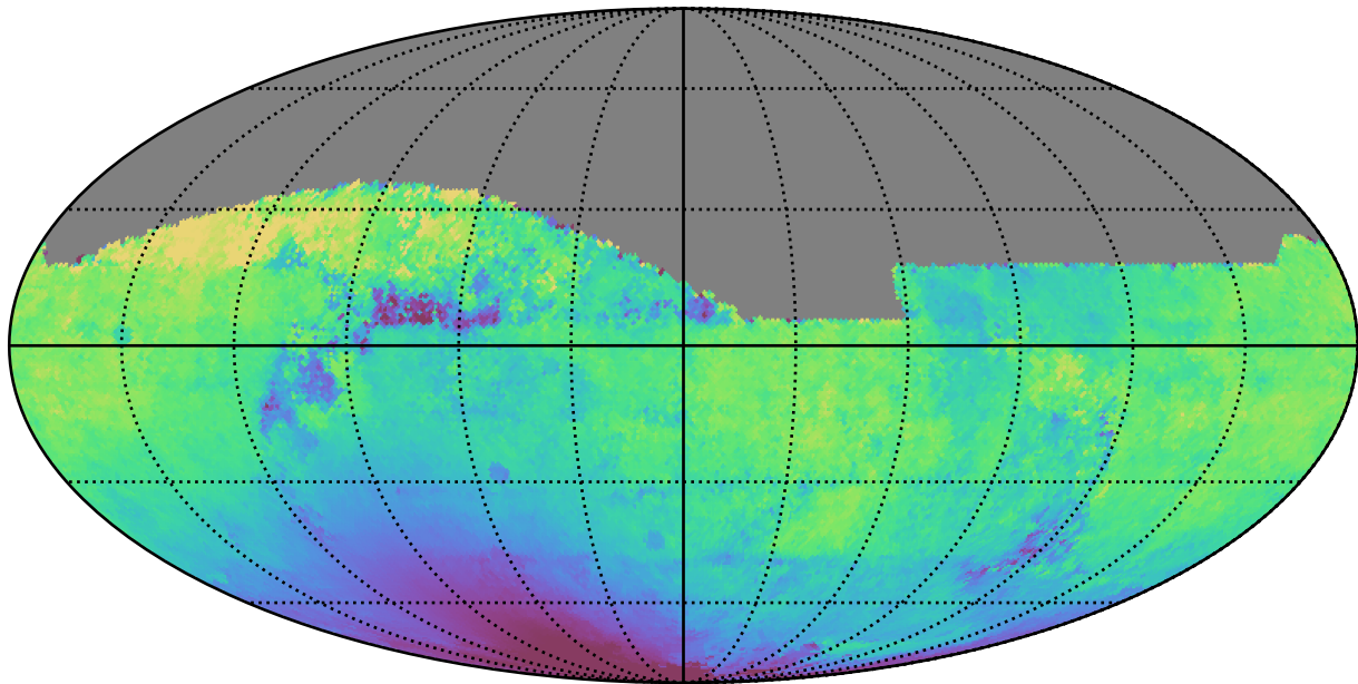
too_elab_r8_d2_gz_v3.4_10yrs All sky z band: Median solarElong
