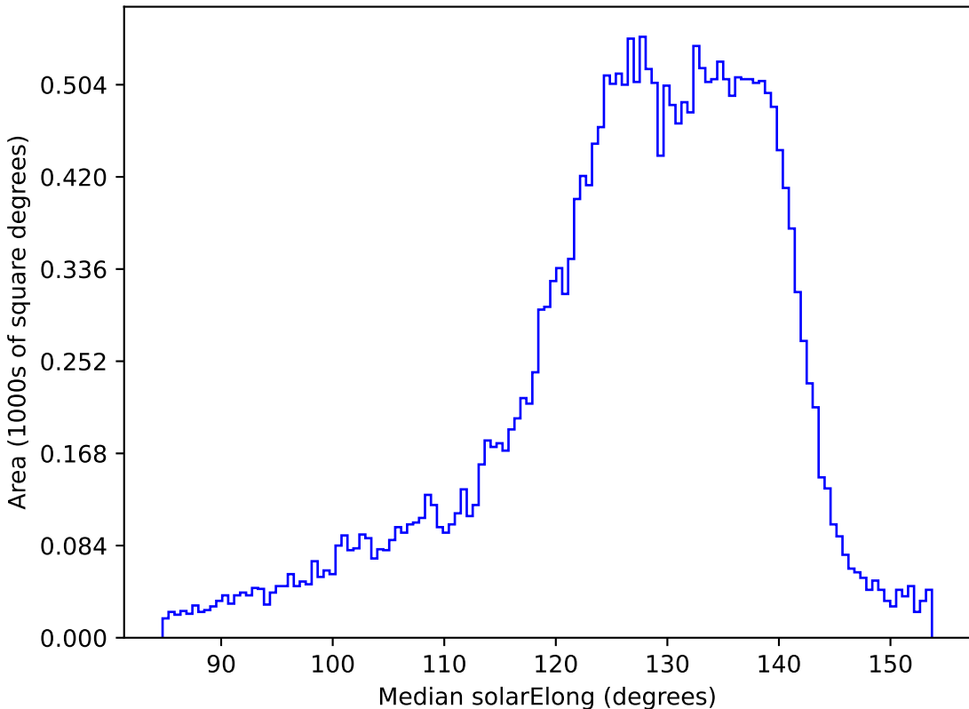
too_elab_r8_d2_gz_v3.4_10yrs All sky z band: Median solarElong
