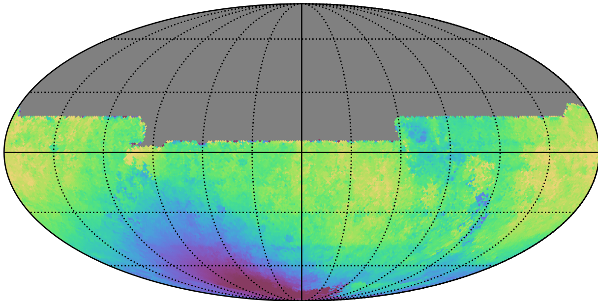
too_elab_r8_d2_gz_v3.4_10yrs All sky y band: Median solarElong
