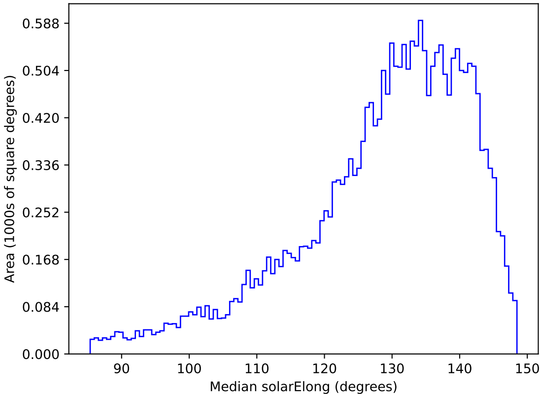
too_elab_r8_d2_gz_v3.4_10yrs All sky y band: Median solarElong
