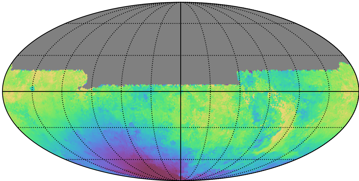
too_elab_r8_d2_gz_v3.4_10yrs All sky u band: Median solarElong
