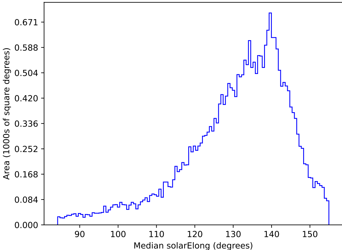
too_elab_r8_d2_gz_v3.4_10yrs All sky r band: Median solarElong
