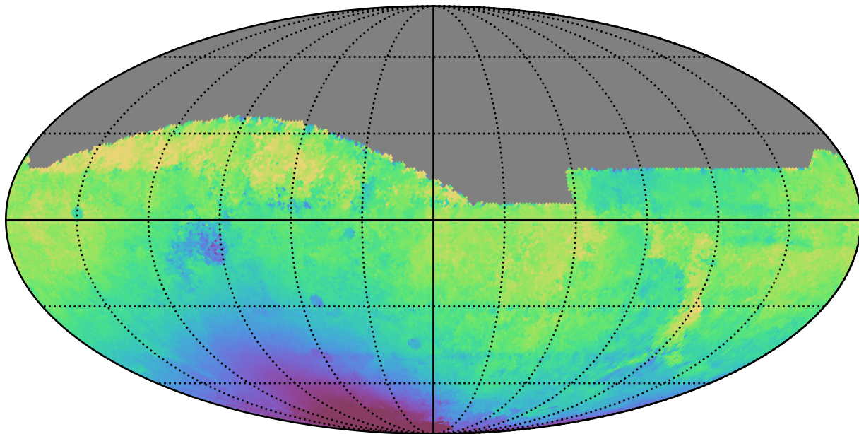
too_elab_r8_d2_gz_v3.4_10yrs All sky i band: Median solarElong
