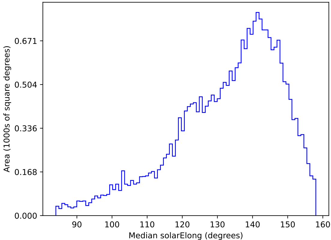
too_elab_r8_d2_gz_v3.4_10yrs All sky g band: Median solarElong
