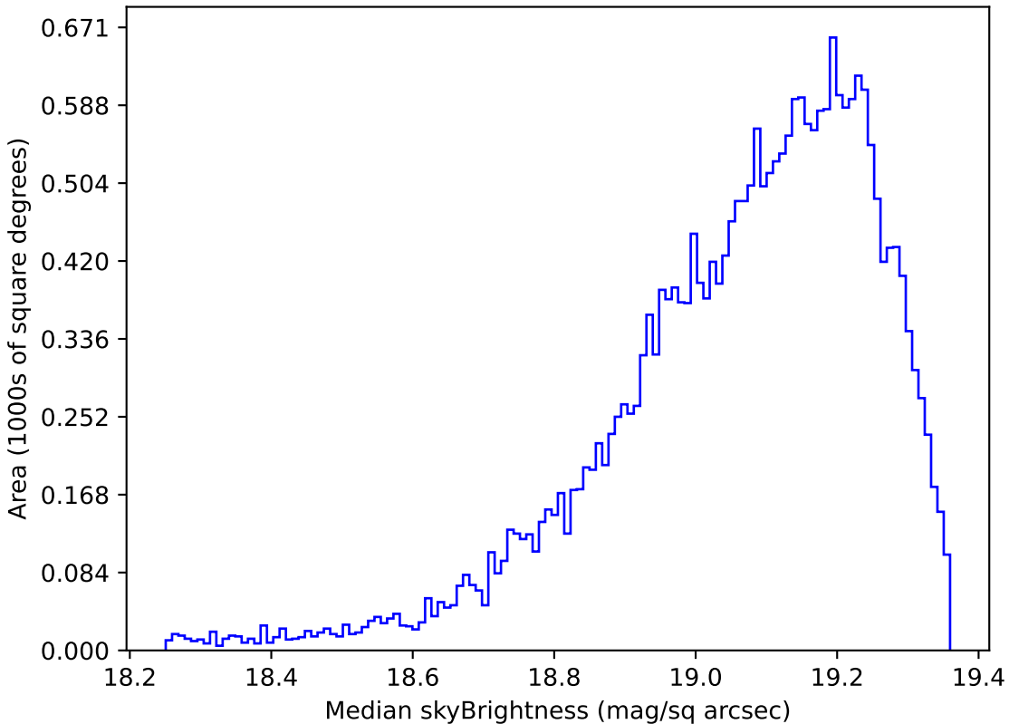
too_elab_r8_d2_gz_v3.4_10yrs Yr 1 z band: Median skyBrightness
