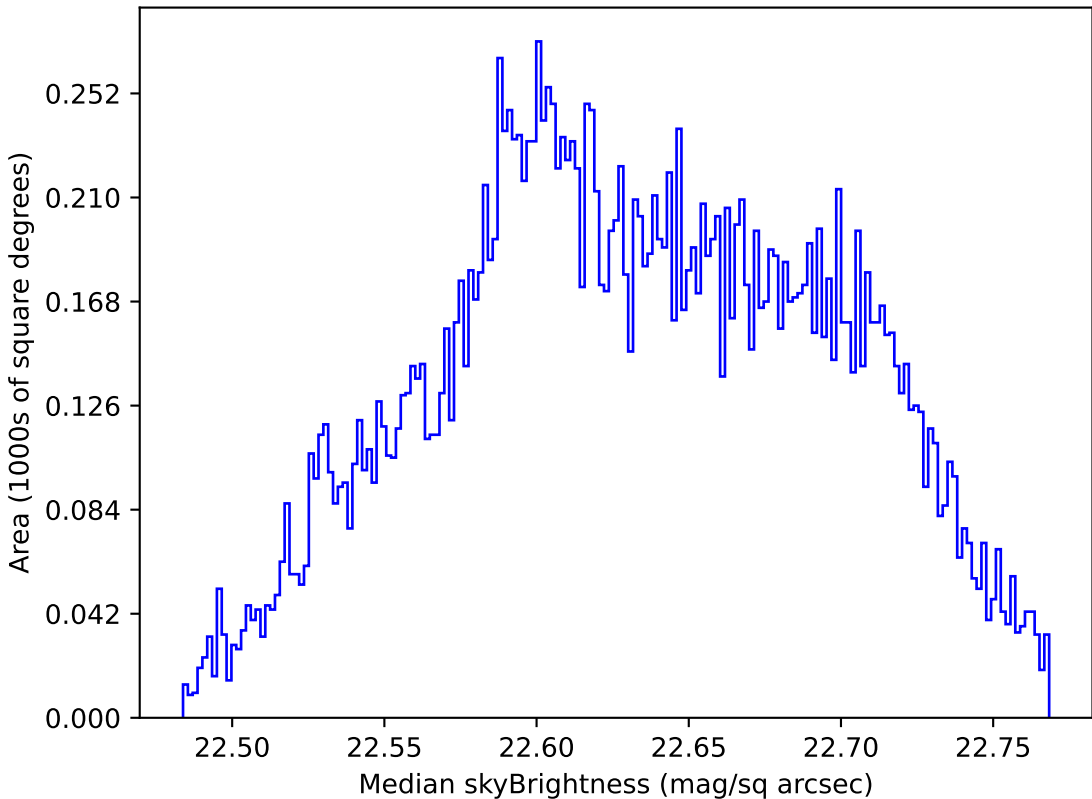
too_elab_r8_d2_gz_v3.4_10yrs Yr 1 u band: Median skyBrightness
