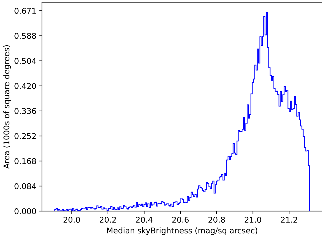
too_elab_r8_d2_gz_v3.4_10yrs Yr 1 r band: Median skyBrightness
