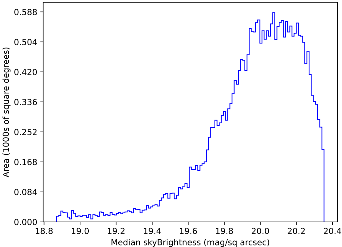
too_elab_r8_d2_gz_v3.4_10yrs Yr 1 i band: Median skyBrightness
