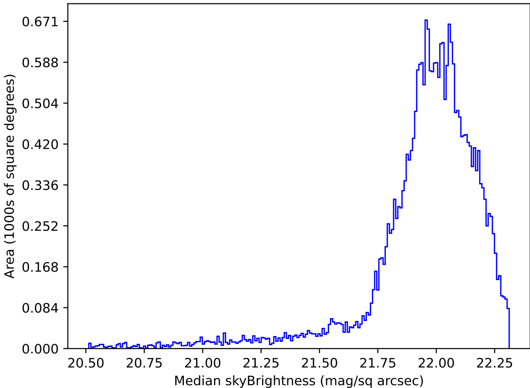
too_elab_r8_d2_gz_v3.4_10yrs Yr 1 g band: Median skyBrightness
