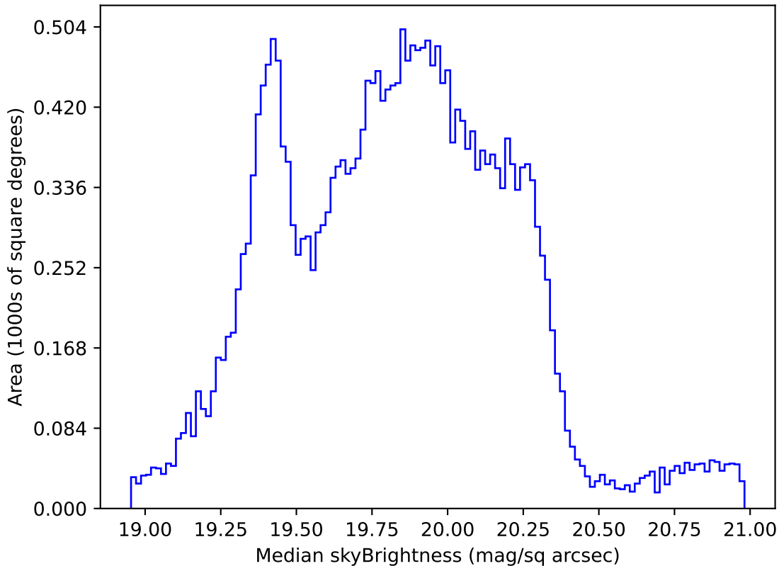
too_elab_r8_d2_gz_v3.4_10yrs Yr 1 all bands: Median skyBrightness
