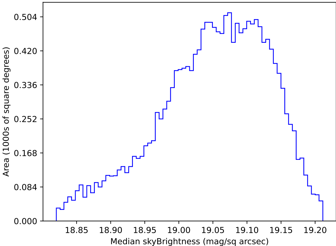
too_elab_r8_d2_gz_v3.4_10yrs WFD z band: Median skyBrightness
